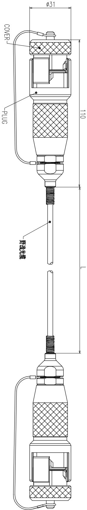
2~4 core plug
